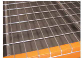
Inverted U-Channel
